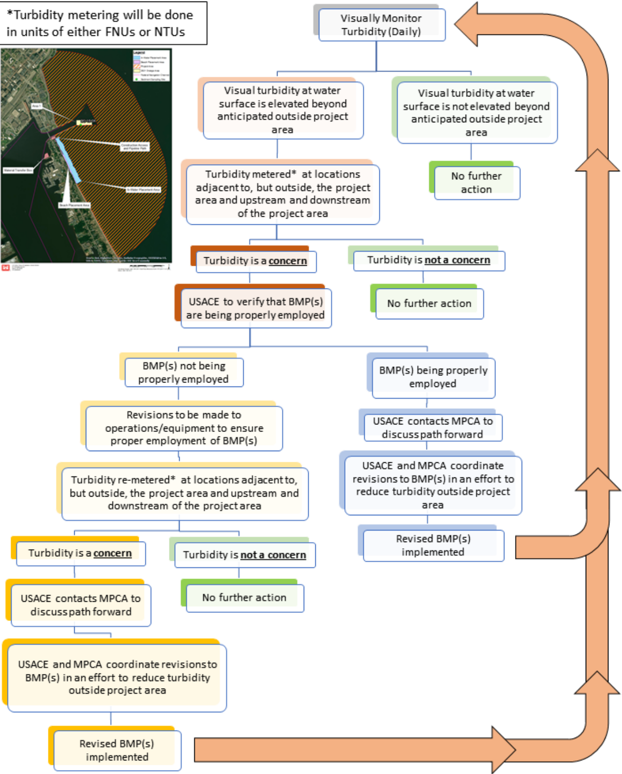
USACE turbidity daily inspection procedure for the Minnesota Point Beach Nourishment Area. Note: the project area limits area shown in the inset and Appendix B, Figures B1 and B2.
